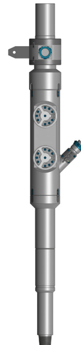
Top Drive Cementing Head CP
