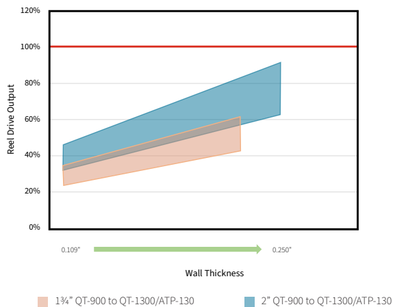
24K Tubing Reel Drive Performance for 1 3/4- and 2-in. Tubing
